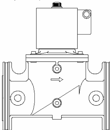
Model VMR8-3"
