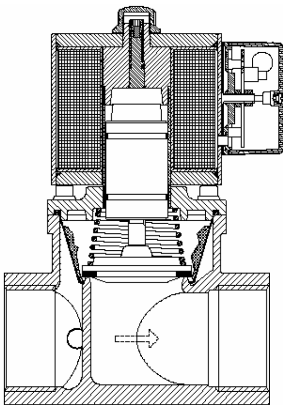
Model VMR6-2"
